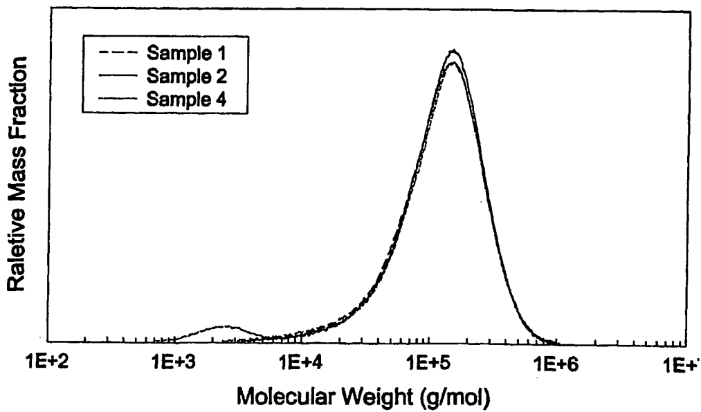
Fig. 14 Molecular Weight Distribution of Plasticized Propylene Homopolymers
